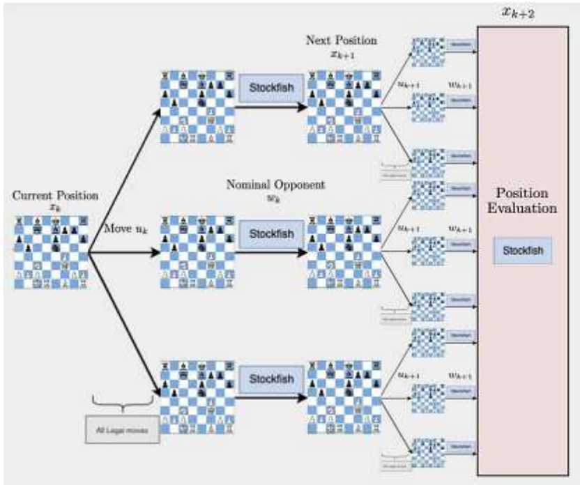
Figure 2.12.2 Illustration of the two-step lookahead version of the computer chess scheme of Fig. 2.12.1. Again we use Stockfish for both opponent move generation and for position evaluation.
