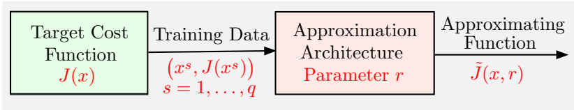
Figure 1.3.5 The general structure for parametric cost approximation. We approximate the target cost function J(x) with a member from a parametric class \tilde{J}(x, r) that depends on a parameter vector r . We use training data (x^s, J(x^s)) , s = 1, \dots, q , and a form of optimization that aims to find a parameter \hat{r} that “minimizes” the size of the errors J(x^s) - \tilde{J}(x^s, \hat{r}) , s = 1, \dots, q .
