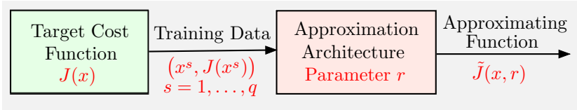
Figure 3.1.1 The general structure for parametric cost approximation. We approximate the target cost function J(x) with a member from a parametric class \tilde{J}(x, r) that depends on a parameter r . We use training data (x^s, J(x^s)) , s = 1, \dots, q , and a form of optimization that aims to find a parameter \hat{r} that “minimizes” the size of the errors J(x^s) - \tilde{J}(x^s, \hat{r}) , s = 1, \dots, q .
