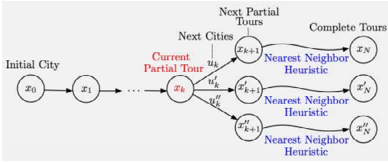
Figure 1.2.9 Rollout with the nearest neighbor heuristic for the traveling salesman problem of Example 1.2.3. The initial state x_0 consists of a single city. The final state x_N is a complete tour of N cities, containing each city exactly once.
