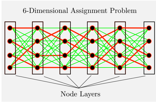
Figure 2.2.1 Illustration of the graph of an (N + 1) -dimensional assignment problem (here N = 5 ). There are N + 1 node layers each consisting of m nodes (here m = 4 ). Each grouping consists of N + 1 nodes, one from each layer, and N corresponding arcs. An (N + 1) -dimensional assignment consists of m node-disjoint groupings, where each node belongs to one and only one grouping (illustrated in the figure with thick lines). For each grouping, there is an associated cost that depends on the N -tuple of arcs comprising the grouping. The cost of an (N + 1) -dimensional assignment is the sum of the costs of its m groupings. The difficulty here is that the cost of a grouping does not decompose into a sum of its N arc costs, so the problem cannot be solved by solving N decoupled 2-dimensional assignment problems (for a suboptimal approach based on enforced decoupling, see [Ber20a], Section 3.4.2).
