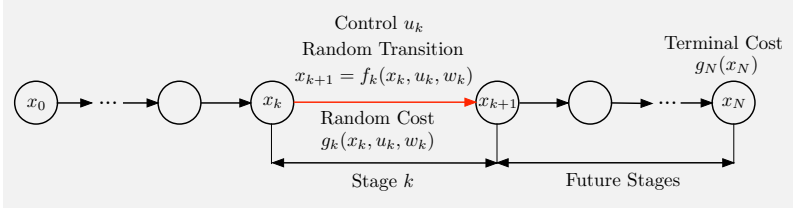
Figure 1.3.1 Illustration of an N -stage stochastic optimal control problem. Starting from state x_k , the next state under control u_k is generated randomly, according to x_{k+1} = f_k(x_k, u_k, w_k) , where w_k is the random disturbance, and a random stage cost g_k(x_k, u_k, w_k) is incurred.
