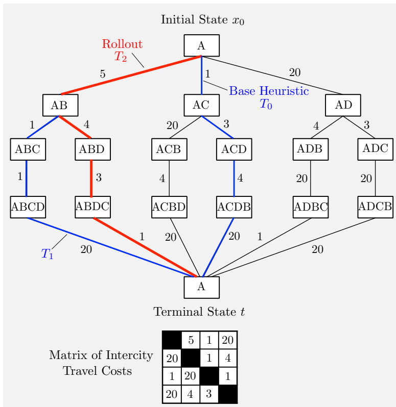
Figure 1.2.10 Rollout with the nearest neighbor base heuristic, applied to a traveling salesman problem. At city A, the nearest neighbor heuristic generates the tour ACDBA (labeled T_0 ). At city A, the rollout algorithm compares the tours ABCDA, ACDBA, and ADCBA, finds ABCDA (labeled T_1 ) to have the least cost, and moves to city B. At AB, the rollout algorithm compares the tours ABCDA and ABDCA, finds ABDCA (labeled T_2 ) to have the least cost, and moves to city D. The rollout algorithm then moves to cities C and A (it has no other choice). The final tour T_2 generated by rollout turns out to be optimal in this example, while the tour T_0 generated by the base heuristic is suboptimal. This is suggestive of a general result: the rollout algorithm for deterministic problems generates a sequence of solutions of decreasing cost under some conditions on the base heuristic that we will discuss in Chapter 2, and which are satisfied by the nearest neighbor heuristic.
