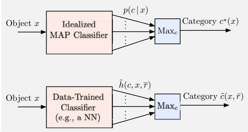
Figure 3.4.1 Illustration of the MAP classifier c^*(x) for the case where the probabilities p(c|x) are known [cf. Eq. (3.34)], and its data-trained version \tilde{c}(x, \bar{r}) [cf. Eq. (3.38)]. The classifier may be obtained by using the data set (x_k^s, u_k^s) , s = 1, \dots, q , and an approximation architecture such as a feature-based architecture or a neural network.
