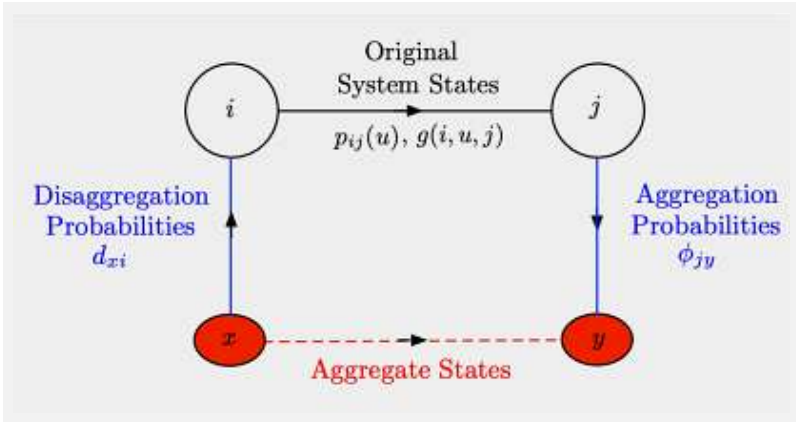
Figure 3.6.6 Illustration of the aggregate system, and the transition mechanism and the costs per stage of the aggregate problem.
