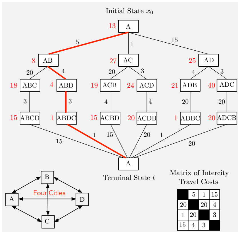
Figure 1.2.7 The DP formulation of the traveling salesman problem of Example 1.2.2. The travel times between the four cities A, B, C, and D are shown in the matrix at the bottom. We form a graph whose nodes are the k -city sequences and correspond to the states of the k th stage, assuming that A is the starting city. The transition costs/travel times are shown next to the arcs. The optimal costs-to-go are generated by DP starting from the terminal state and going backwards towards the initial state, and are shown next to the nodes. There is a unique optimal sequence here (ABDCA), and it is marked with thick lines. The optimal sequence can be obtained by forward minimization [cf. Eq. (1.8)], starting from the initial state x_0 .
