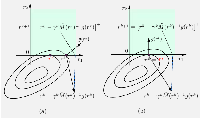
Figure 3.5.2. Two-dimensional examples where I^+(r_k) = \{2\} [we have r_1^k > 0 , while r_2^k = 0 and g_2(r^k) > 0 ]. The iteration is r^{k+1} = [r^k - \gamma^k \tilde{M}(r^k)^{-1} g(r^k)]^+ . (a) A case where the iteration fails to make progress when \tilde{M}(r^k) is not properly diagonalized. (b) A case where the iteration fails to stop at an optimal solution r^* when \tilde{M}(r^k) is not properly diagonalized.
