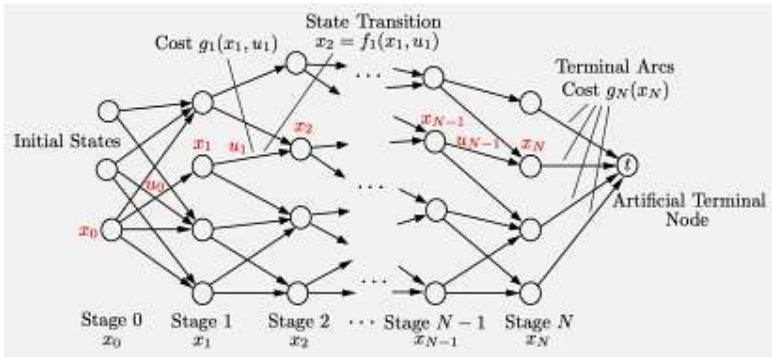
Figure 2.1.2 Illustration of a deterministic finite-state DP problem. Nodes correspond to states x_k . Arcs correspond to state-control pairs (x_k, u_k) . An arc (x_k, u_k) has start and end nodes x_k and x_{k+1} = f_k(x_k, u_k) , respectively. The cost g_k(x_k, u_k) of the transition is the length of this arc. An artificial terminal node t is connected with an arc of cost g_N(x_N) with each state x_N . The problem is equivalent to finding a shortest path from initial nodes of stage 0 to node t .
